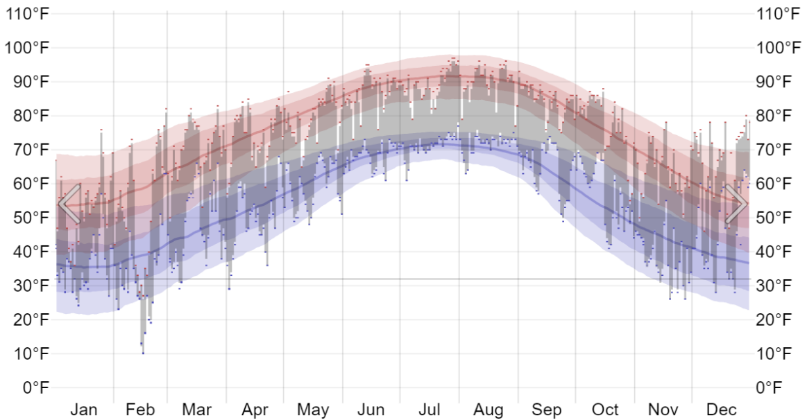
Hourly Temperature in 2021 in Starkville
